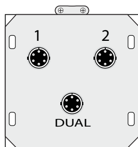
Junction Box Cover with 3 Female 6-pin Connectors
